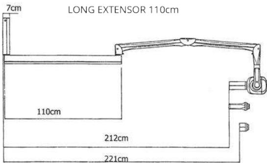
BRACKET 1.10m
